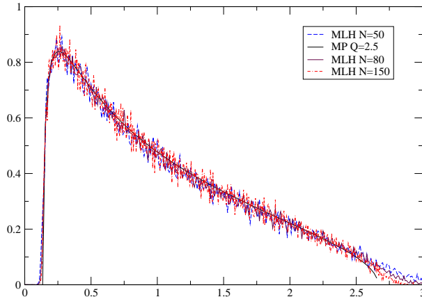
FIG. 2: Comparison between the numerical solution of the self-consistent equation (12) for N = 50, 80, 150 and Q = 2.5 (500 samples) and the Marčenko-Pastur distribution. The agreement is excellent. Notice that the blurring of the MP right edge is a finite size effect, as shown by the evolution from N = 50 to N = 150 .
