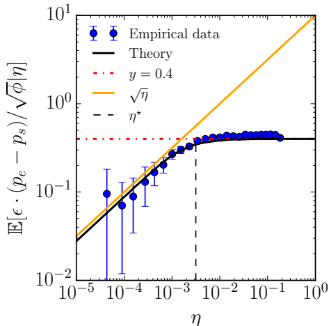
FIG. 1. Empirically determined scaling function \mathcal{F}(\eta) vs. participation rate \eta . The data (blue points) interpolates between a \sqrt{\eta} behaviour observed at small participation rates and an asymptotically constant regime \approx 0.4 for large \eta , i.e. for \eta \gtrsim \eta^* with \eta^* \approx 3.15 \times 10^{-3} . Black line: prediction of LLOB, with an adjusted crossover \eta^* := J_s/J_f allowing for the existence of two categories of agents (“fast” and “slow”). The data points are obtained by restricting to metaorders with sufficient large order size, i.e. \phi \gtrsim 10^{-5} .
