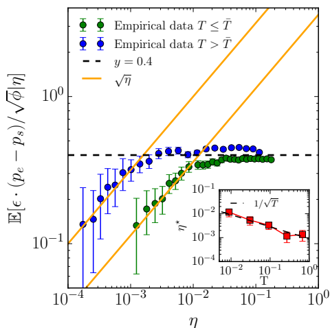
FIG. 2. (Main panel) Empirically determined scaling function \mathcal{F}(\eta) vs. participation rate \eta for metaorders with duration T larger (blue dots) or smaller (green dots) than the median sample duration \bar{T} \approx 0.09 . Note that the crossover value \eta^* is \sim 10 times larger in the latter case. Note that the asymptotic value of \mathcal{F} (and hence the impact for a given Q ) is approximately independent of T , as predicted by the theory. Both empirical curves are obtained using metaorders with sufficient large order size, i.e. \phi \gtrsim 10^{-5} . (Inset) Plot of the crossover participation rate \eta^* as a function of the execution time T , revealing an approximate T^{-1/2} behaviour.
